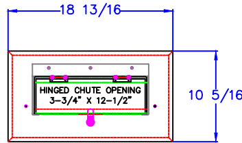
FRONT VIEW SHOWN WITH PAIRED SS SLEEVE
